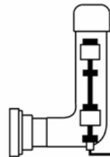
WATER LEVEL SENSOR ASSY: Allows the controls system to monitor the water level inside the Saptistry. May be a float or pressure switch device.
